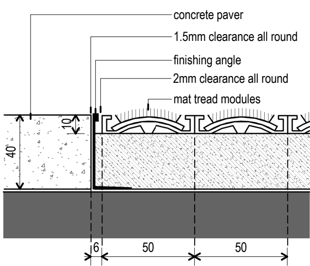
5 Transition Paver/Entry Mat 1 : 2
