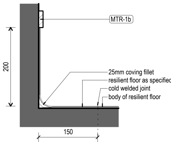
6 Skirting - Covered Vinyl 1 : 5
