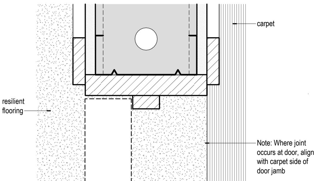
9 Transition - Resilient Floor/Carpet Floor Plan 1 : 2 AS 1428.1 compliant
