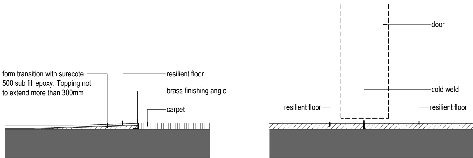
3 Transition Resilient Floor/Carpet 1 : 2 AS 1428.1 compliant
