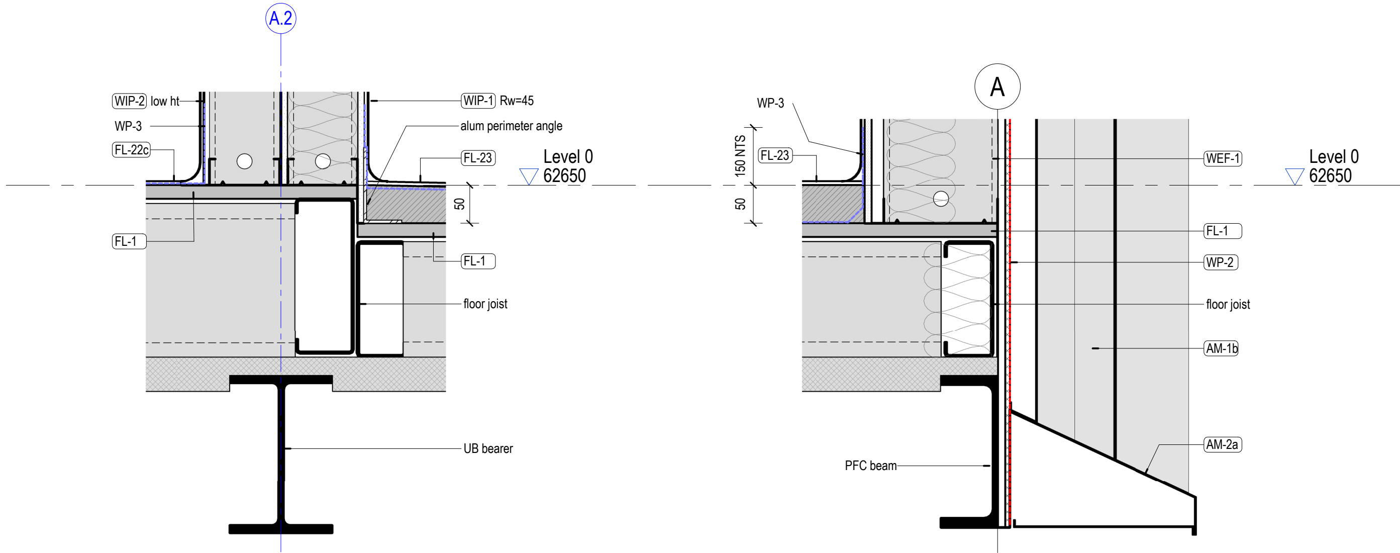
1 Wet Area Floor Setdown 1 : 5 Typ. Internal Wall
