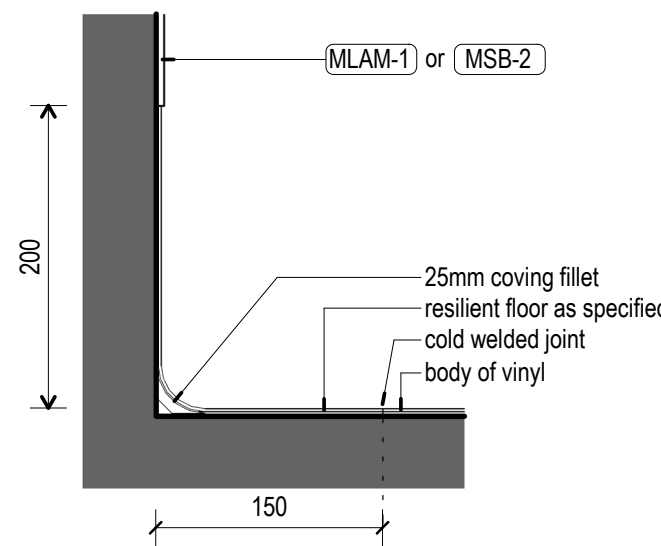
7 Skirting - Covered Vinyl 1 : 5
